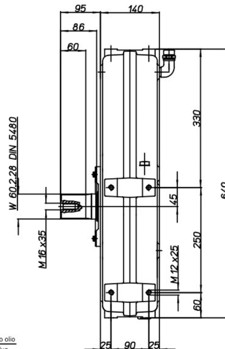
TMP 350 Dimensions
